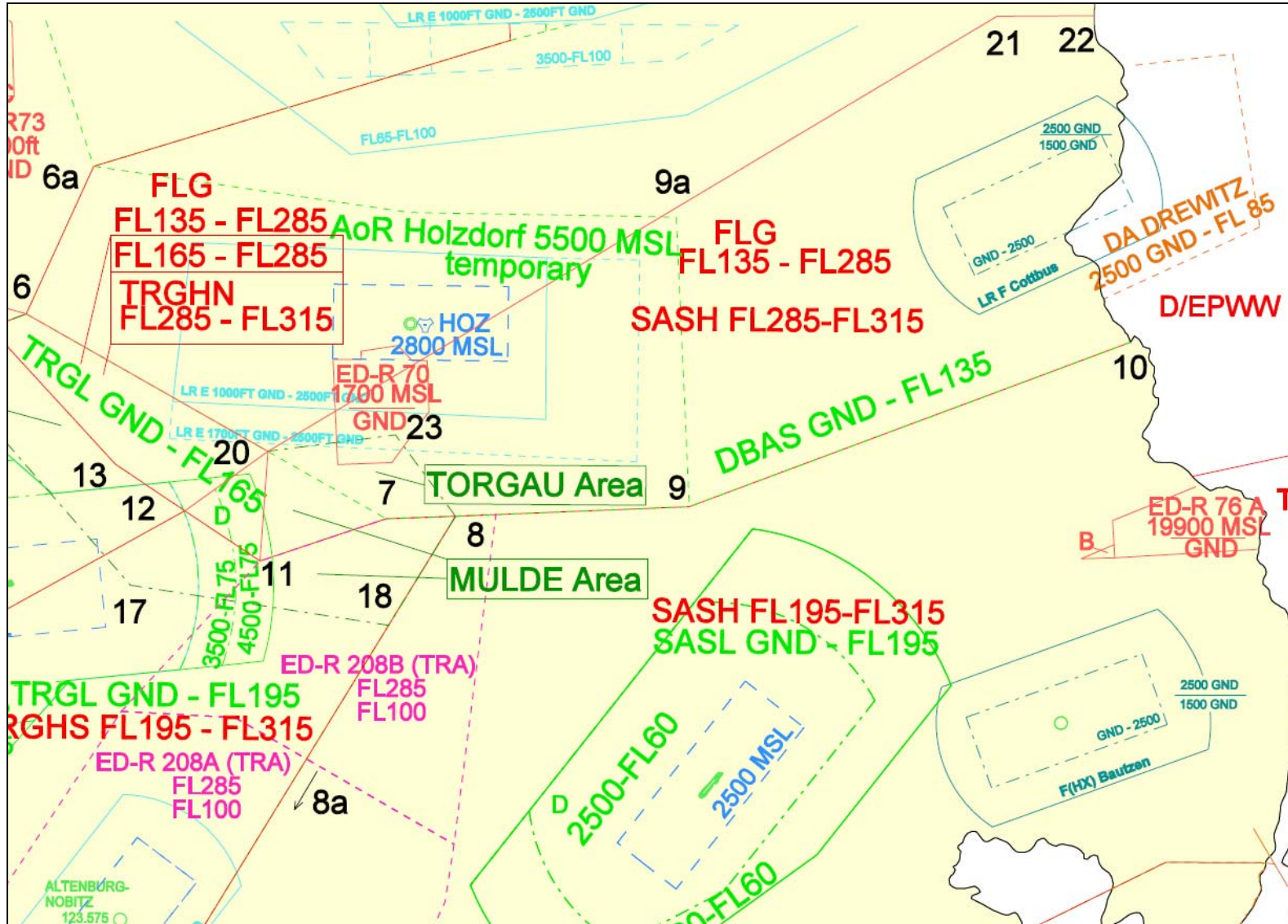
Chart 2 Sectorisation close to the AOR boundary of Munich and Bremen ACC, eastern part.
