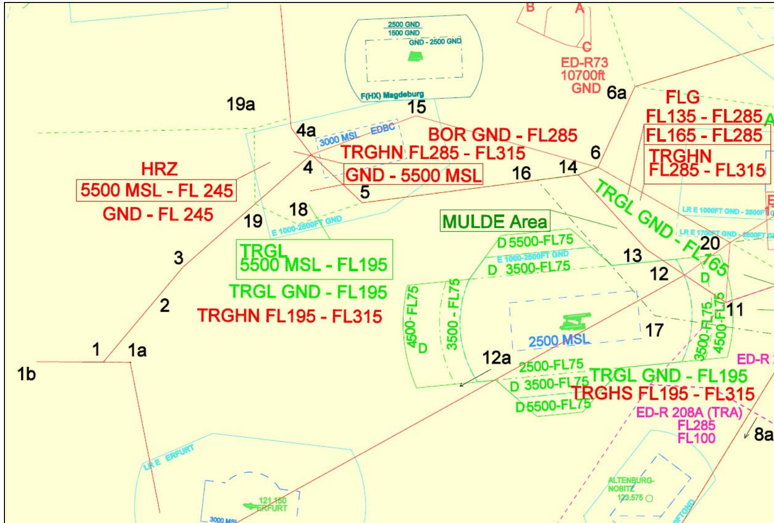
Chart 1 Sectorisation close to the AOR boundary of Munich and Bremen ACC, western part.
